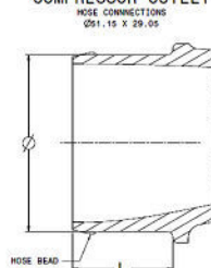
COMPRESSOR OUTLET HOSE CONNECTIONS Ø51.15 X 29.05
