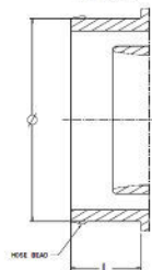
COMPRESSOR INLET HOSE CONNECTIONS Ø51.2 X 28.40
