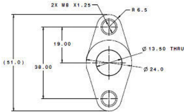
OIL OUTLET
