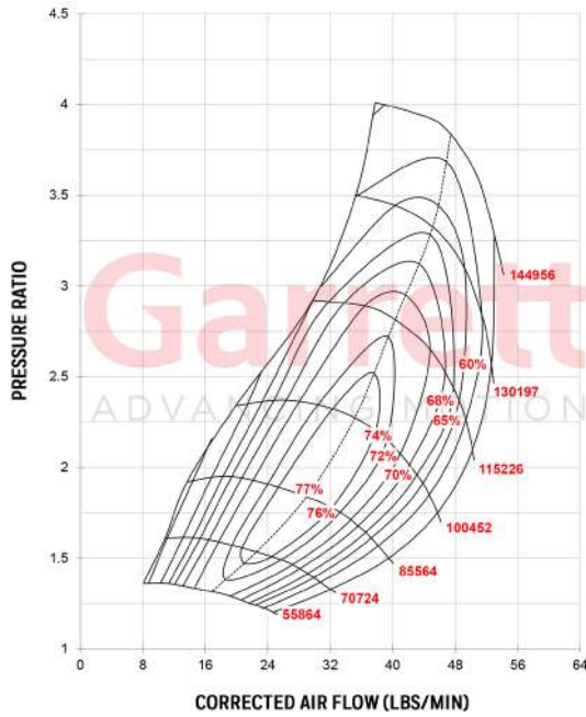
COMPRESSOR MAP
