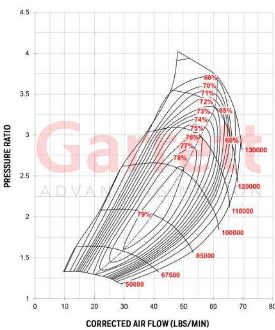
COMPRESSOR MAP
