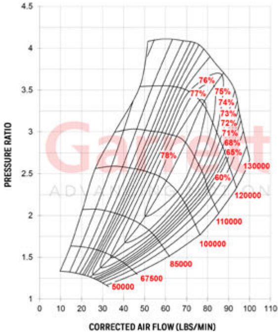
COMPRESSOR MAP
