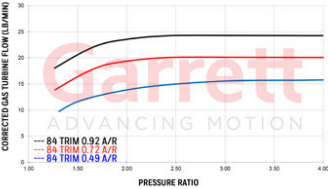
EXHAUST FLOW CHART
