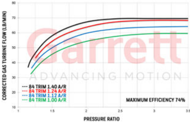
EXHAUST FLOW CHART
