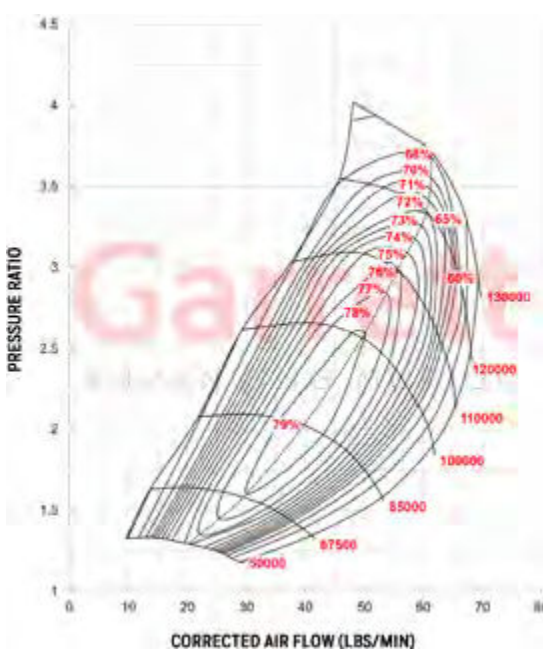
COMPRESSOR MAP
