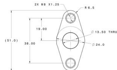
OIL OUTLET
