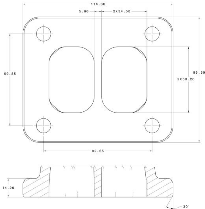
TURBINE INLET T4 BOLTED CONNECTIONS
