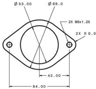
Compressor Inlet
