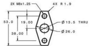
18 Oil Outlet
