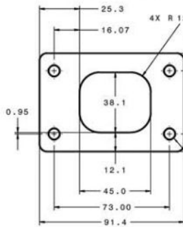
02 Turbine Inlet "T25 WITH STUDS"
