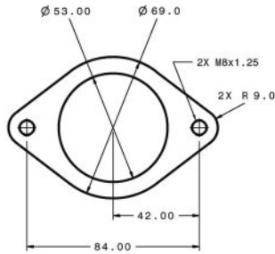
Compressor Inlet
