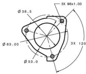
Compressor Outlet
